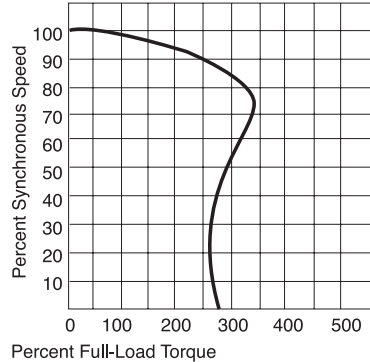
Breakdown Torques by Horsepower
