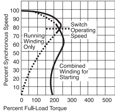
FH High Starting Torque Split Phase
