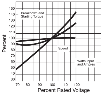
Voltage Variation Effects
