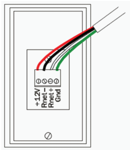
Fig. 9 - Typical Rnet Communication Sensor Wiring
