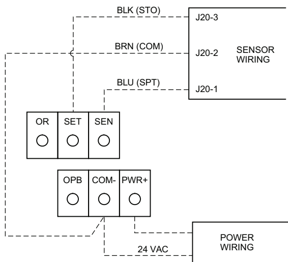
Fig. 6 - Space Temperature Sensor Typical Wiring (33ZCT56SPT)
