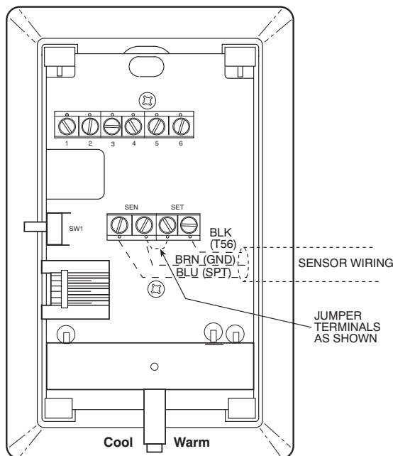
Fig. 6 - Space Temperature Sensor Typical Wiring (33ZCT56SPT)
