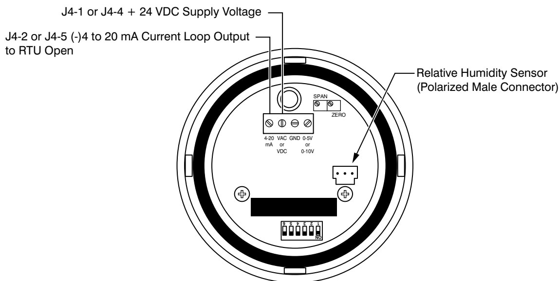
Fig. 12 - Duct Relative Humidity Sensor Typical Wiring
