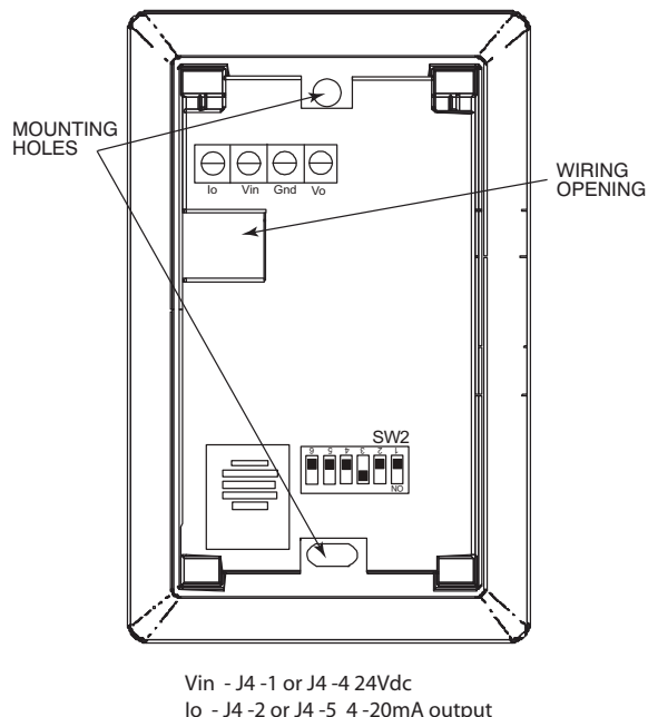
Fig. 11 - Space Relative Humidity Sensor Typical Wiring
