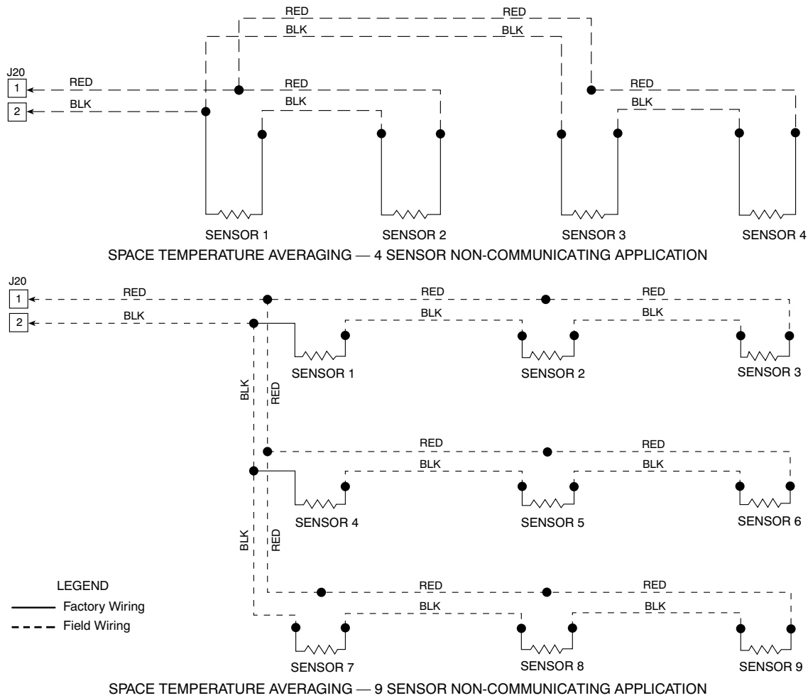
Fig. 8 - Space Temperature Averaging for Non-Communicating Sensors
