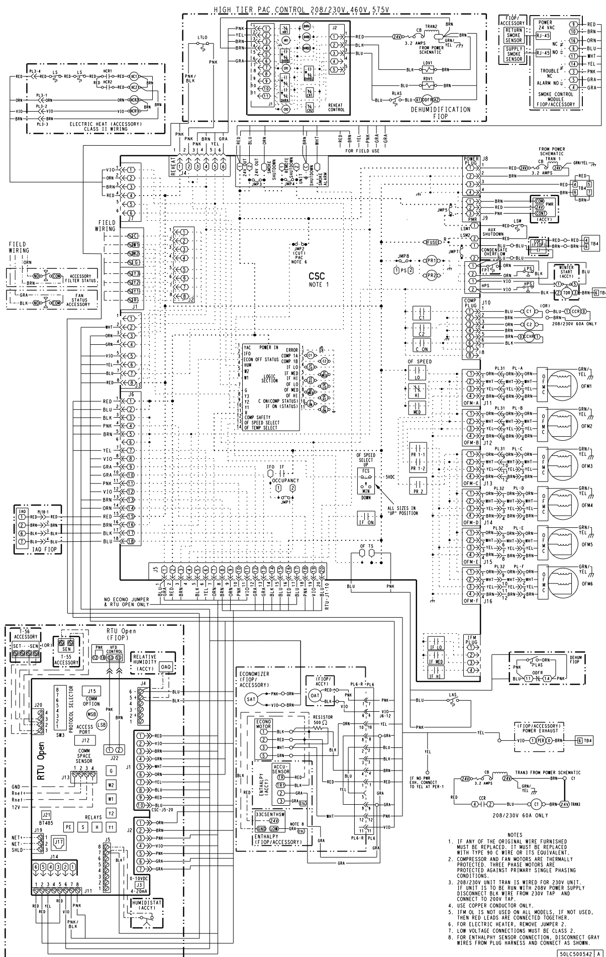
Fig. 2 - Typical Factory Option Wiring - 50LC 14-26 Shown
