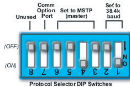
Fig. 14 - RTU Open SW3 Dip Switch Settings
